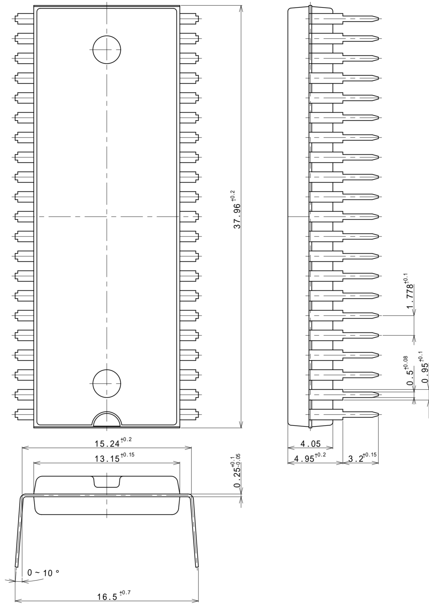
SHDIP42P(600mil)
